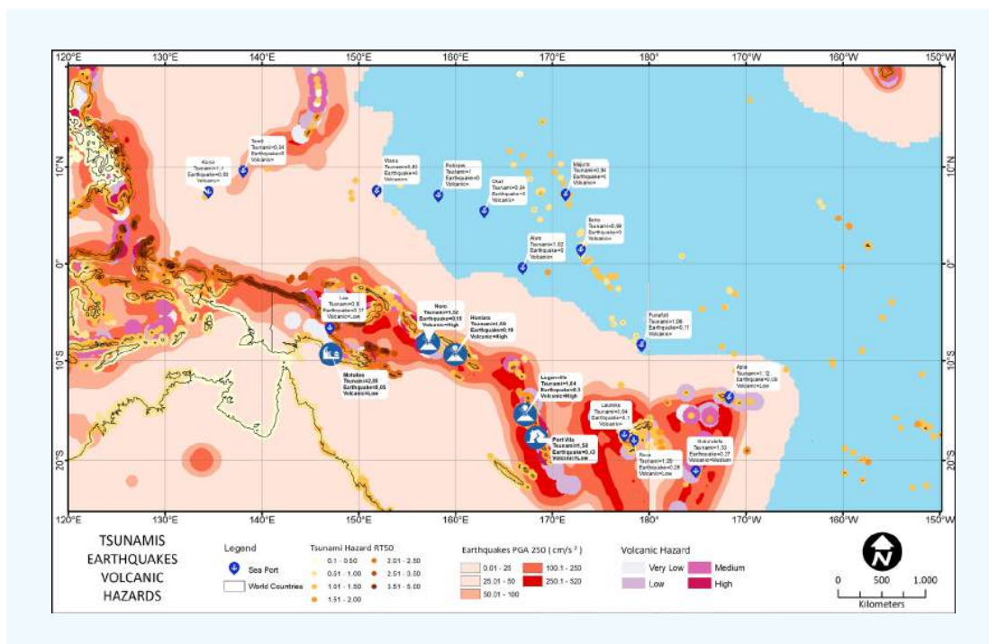
➤ Figure 17: Multi-hazard maps for: (a) Tsunami Hazard Rupug; (b) Earthquake Peak Ground Acceleration (250 year return period); and (c) Volcanic Hazard Level (VHL).
