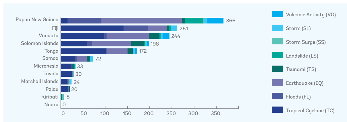
► Figure 15: Total Natural Hazard Events Recorded from 1900–2020, by Country
