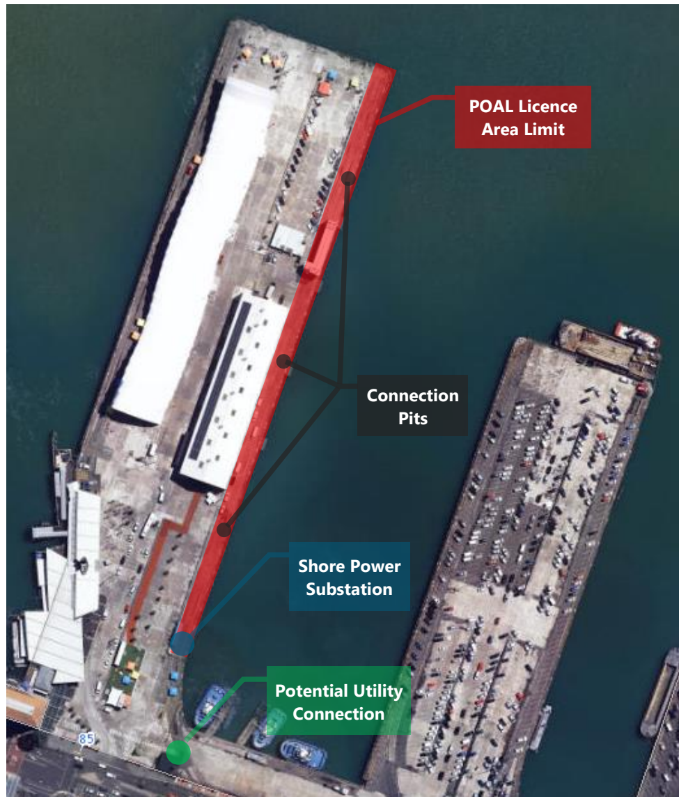
Figure 4-2 POAL Assumed Shore Power Layout
