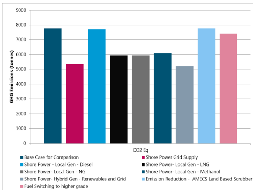
Figure 5-4 Annualised GHG Emission Levels in Year 1 (33% Vessels using Shore Power)
