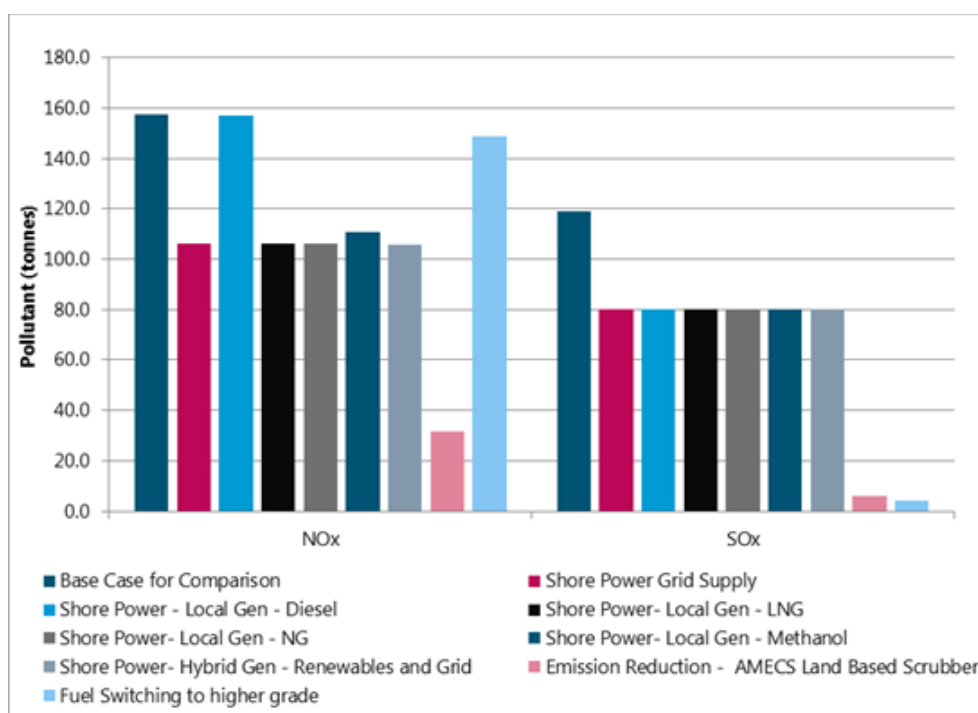
Figure 5-2 Annualised Pollutant NOx and SOx Emission Levels for Year 1 (33% Vessels using Shore Power)
