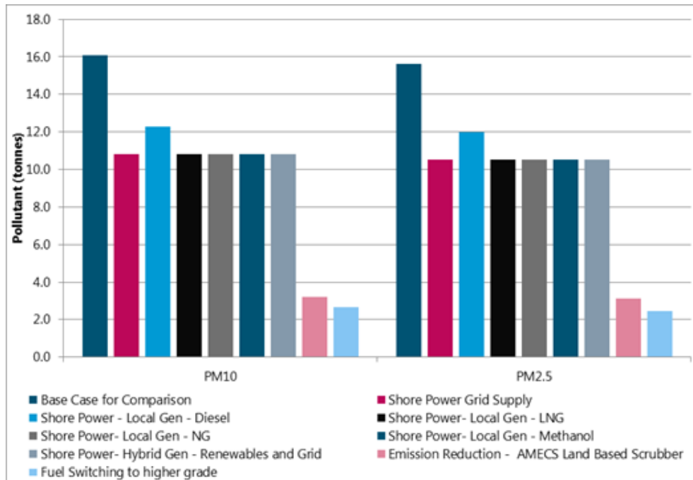
Figure 5-3 Annualised Pollutant PM 10 and PM 2.5 Emission Levels for Year 1 (33% Vessels using Shore Power)
