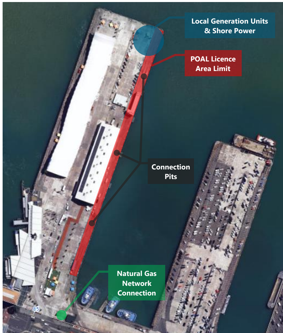
Figure 4-3 POAL Shore Power Local Generation layout
