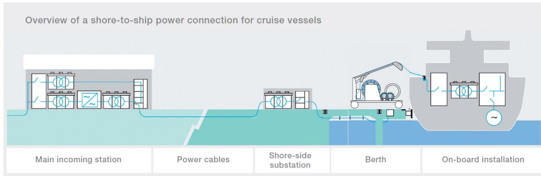
Figure 4-1 Typical Shore Power Connection (ABB, 2016)
