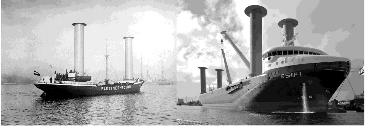
Figure 1: One of the first rotor ships, the Buckau (left), and the present-day rotor ship E-Ship 1 (right)
