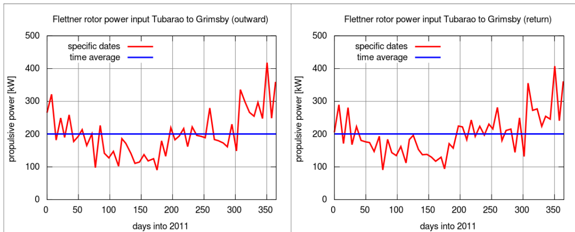
Figure 2: Average power contribution from the Flettner rotor along the route Tubarao to Grimsby, at 53 different times in 2011 (red), and average over all times (blue). Left: Journey from Tubarao to Grimsby. Right: Return journey from Grimsby to Tubarao.
