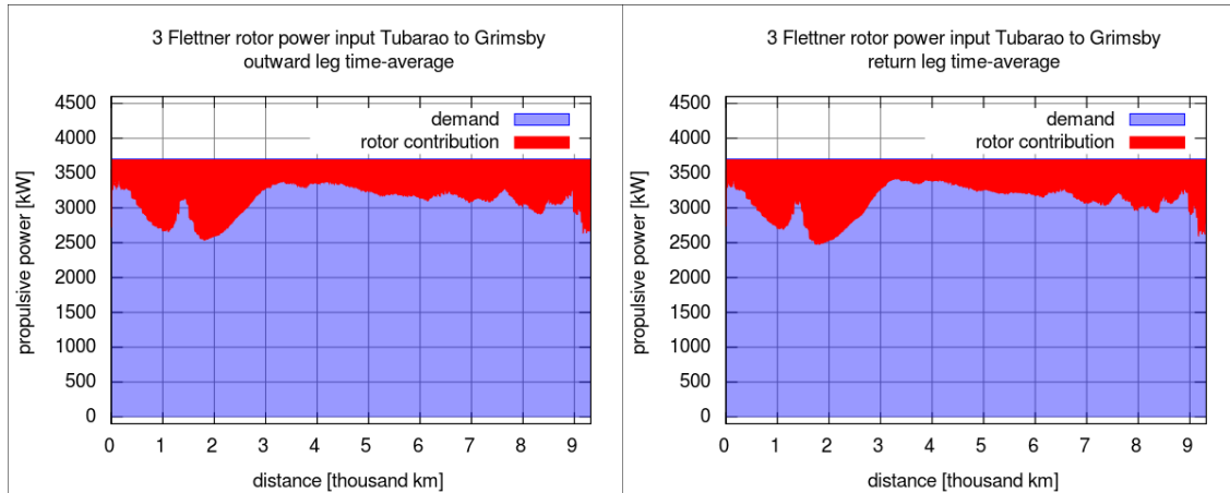
Figure 3: Time-averaged propulsive power generated by a set of three Flettner rotors, plotted as a share of the main engine power requirement of a slow-steaming, 50,000 dwt bulk carrier (cf. section 2.1 and 2.2). Left: On the way from Tubarao to Grimsby. Right: Returning from Grimsby to Tubarao.
