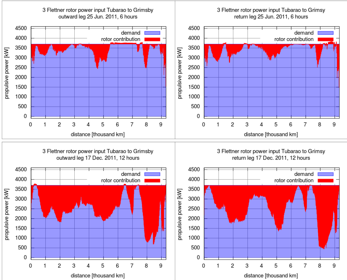
Figure 4: Propulsive power generated by a set of three Flettner rotors, as a share of the main engine power requirement of a slow-steaming, 50,000 dwt bulk carrier (cf. section 2.1 and 2.2). Top: on 25 June 2011, at 6 h, when the wind power contribution was lowest. Bottom: on 17 December 2011, at 12 h, when wind power contribution was highest (out of all 53 datasets). Left: On the way from Tubarao to Grimsby. Right: Returning from Grimsby to Tubarao.
