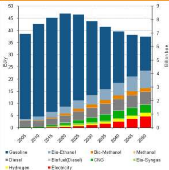
Figure 22 Fuels for LDV cars (a) Demand between 2010 and 2050
