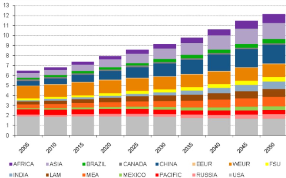
Figure 21 Total transport CO 2 emissions (GtCO 2 /y)
