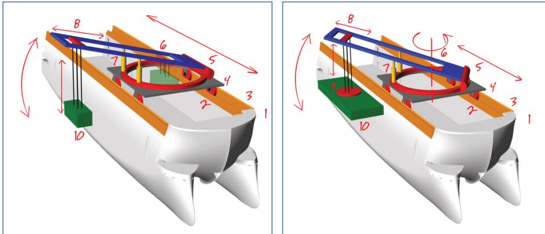
Fig. 4a: New onboard Crane working in Gantry-mode. Source: ILCX
