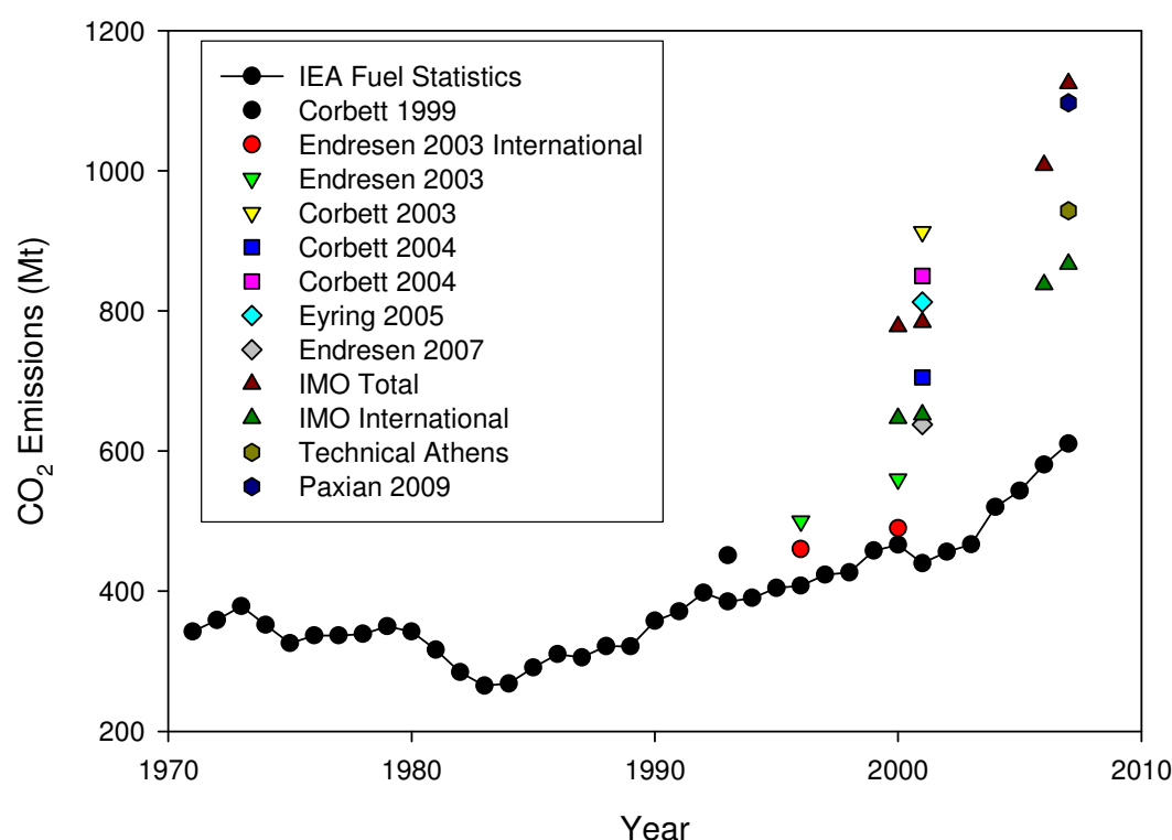
Figure 1-3: Estimated CO 2 release for total and international shipping emissions
