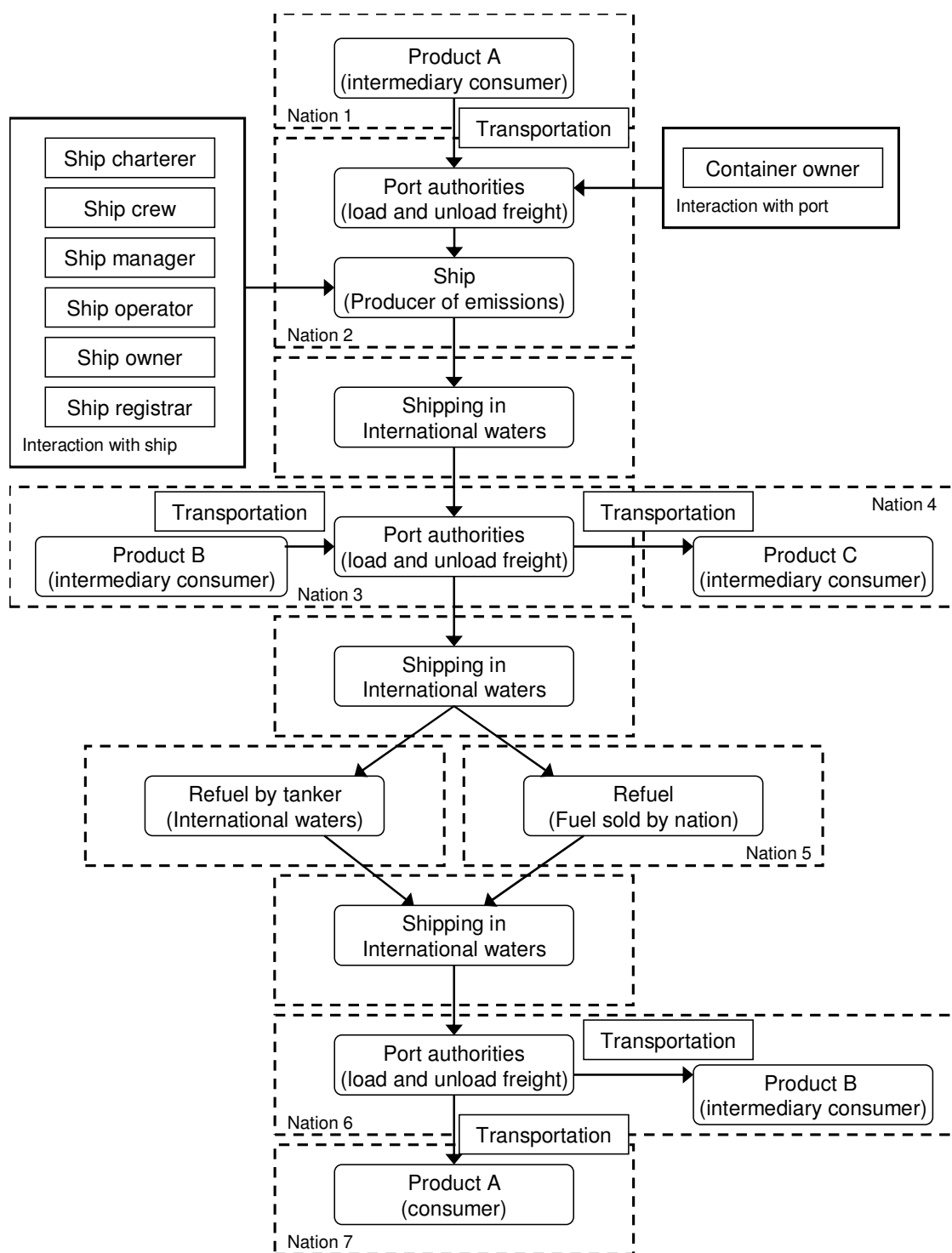
Figure 1-2: A schematic of the shipping system: an example for the shipping of goods between two landlocked nations highlighting the complex nature of shipping
