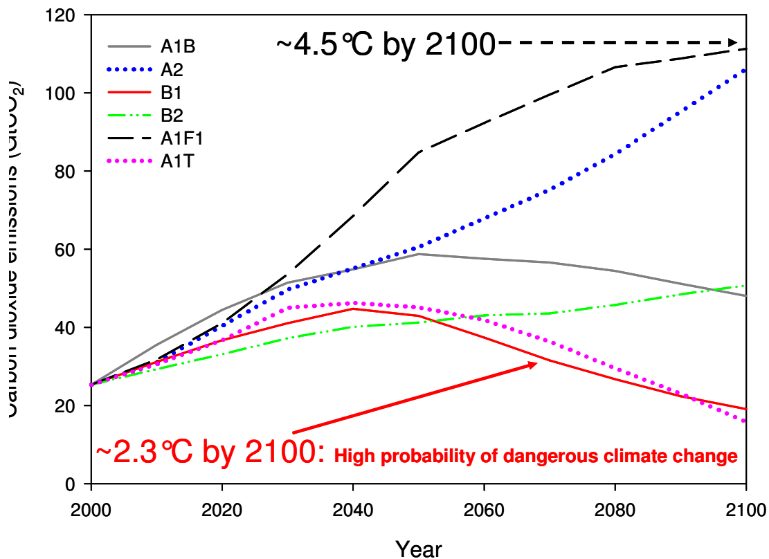
Figure 3-2: IPCC SRES global cross-sector emission scenarios
