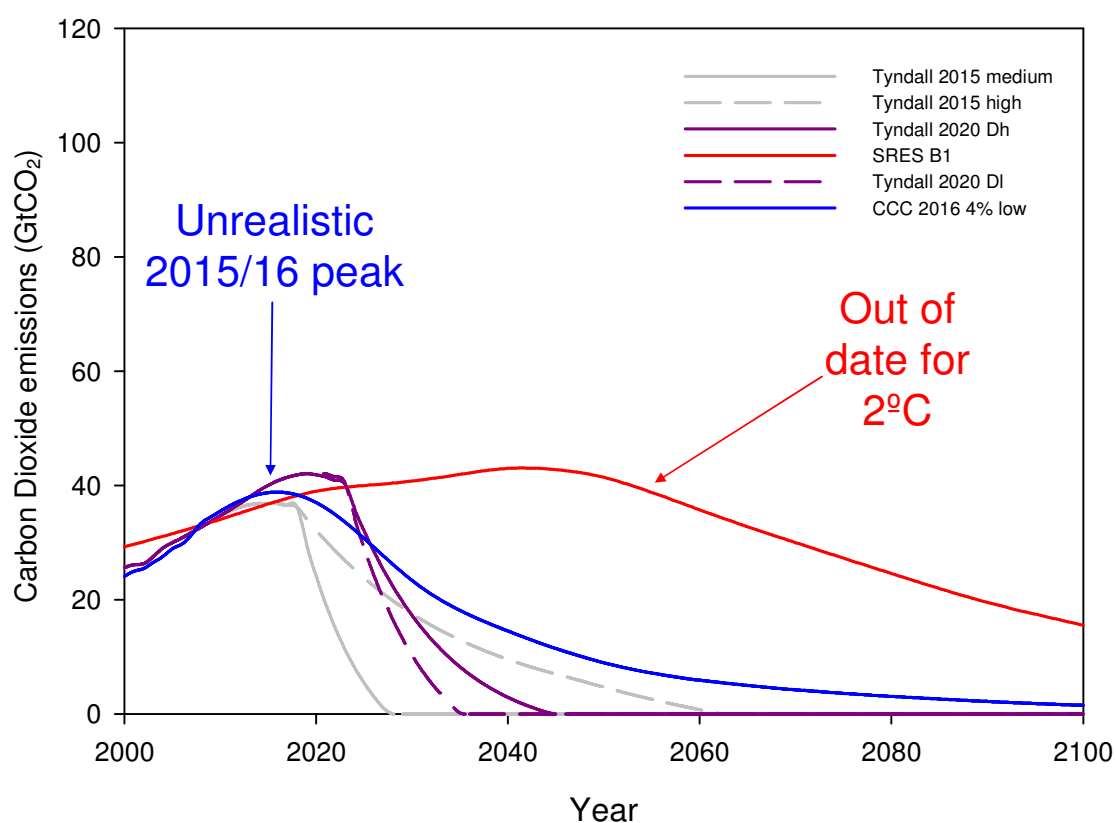
Figure 3-5: Emission scenarios from the three sets presented in Figure 3-2 to Figure 3-4 selected for their relatively low future climate impacts
