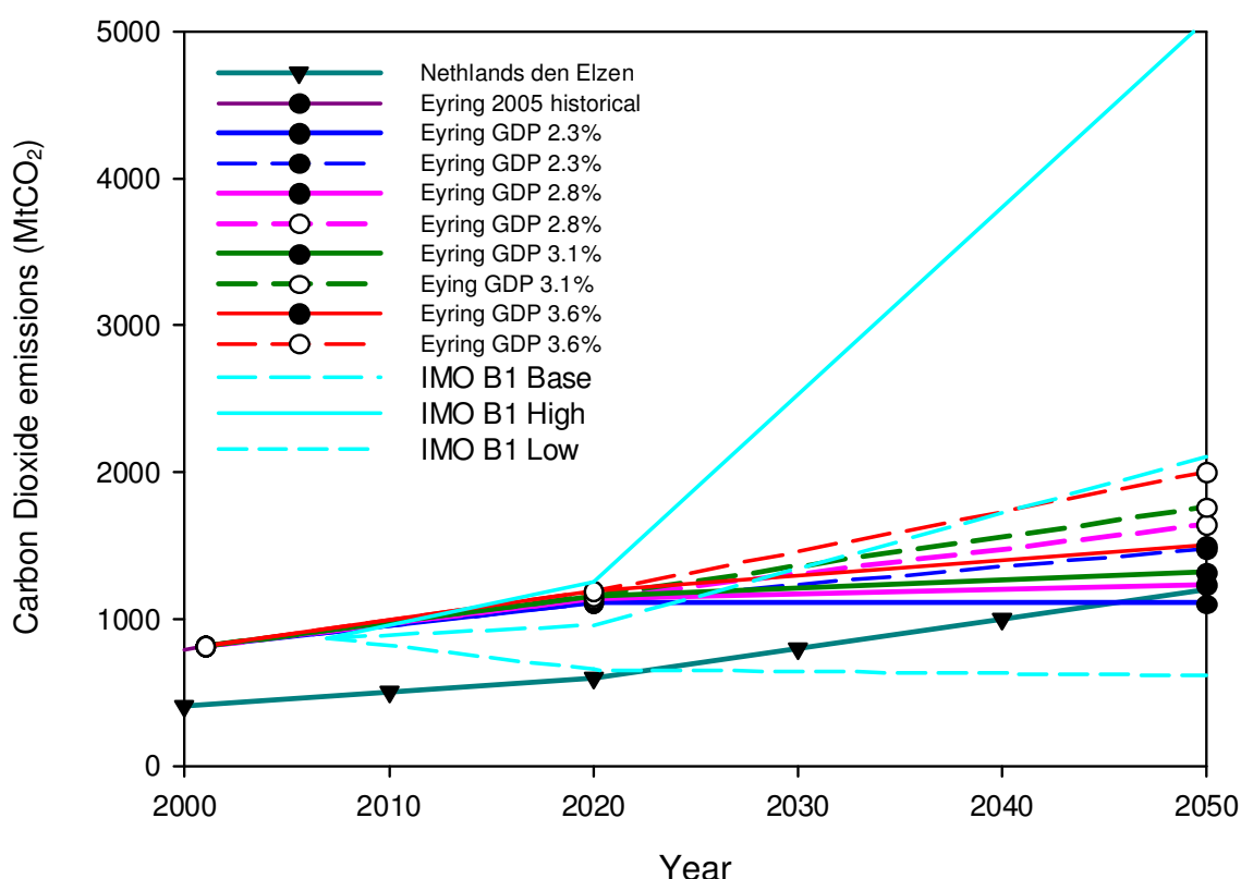
Figure 3-6: Global CO 2 emission projections/scenarios for the shipping sector (Eyring et al. 2005b; IMO 2009)
