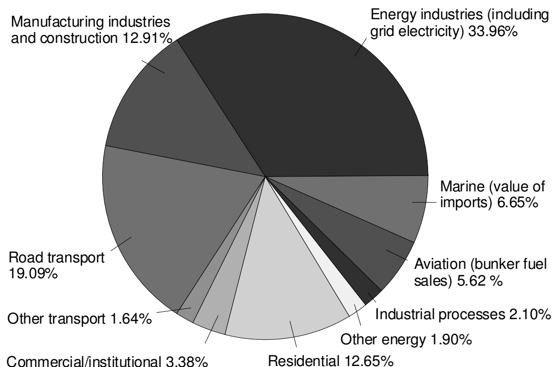
Figure 1-4: UK sector split of CO 2 emissions, apportioning international shipping emissions using bunker fuel sold and value of UK imports
