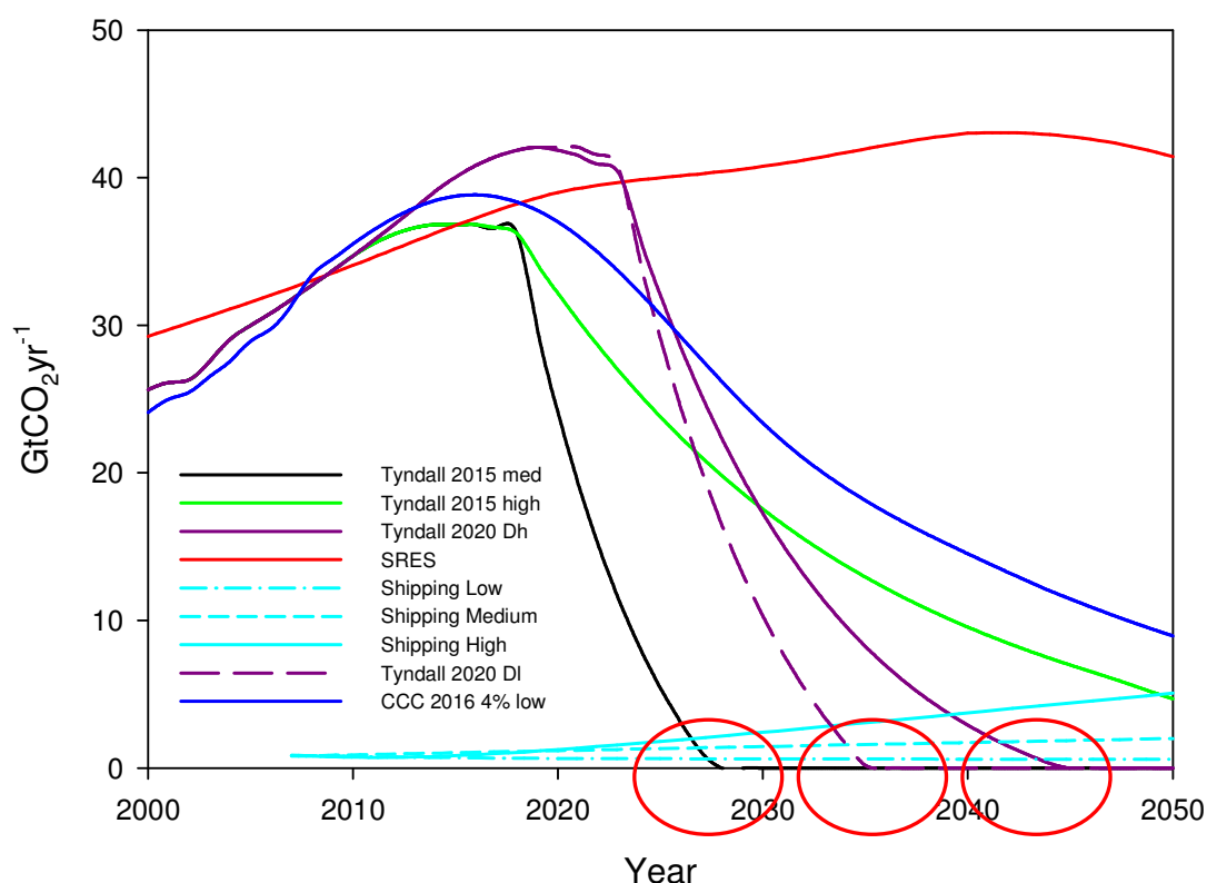
Figure 3-7: Comparison of a selection of low, medium and high emission scenarios for shipping with global 2°C emission scenarios
