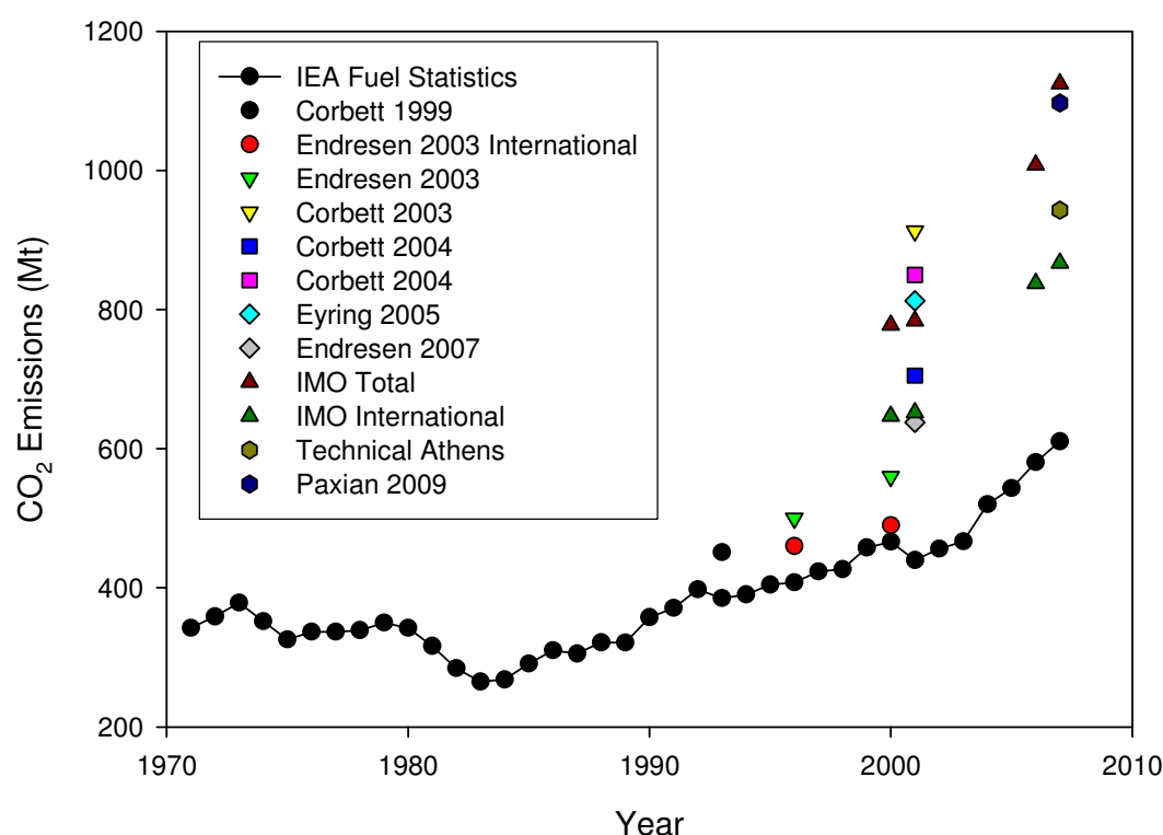
Figure 5-1: Estimated CO 2 release for total and international shipping emissions
